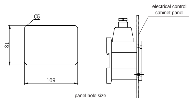
Cover Mounting
