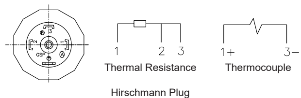
Hirschmann Plug
