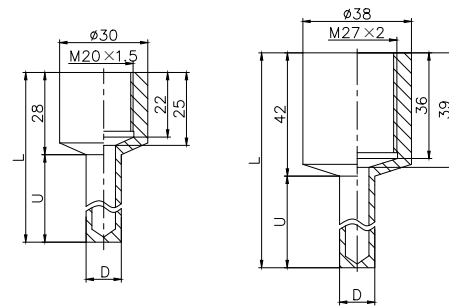
Welding Sleeving
