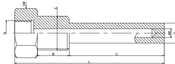
Threaded Installation Sleeving
