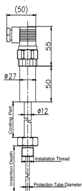
Hirschmann Plug
