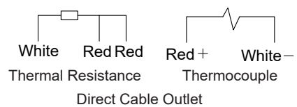
Direct Cable Outlet
