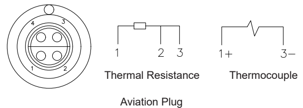
Aviation Plug
