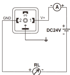
2-wire 4mA ~ 20mA Output
