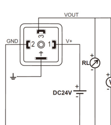
3-wire Voltage Output
