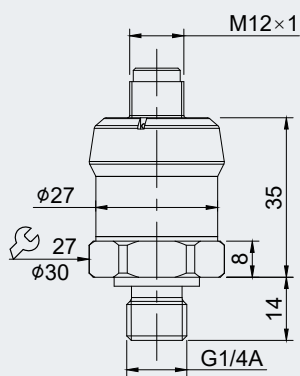
M12×1(4-pin) Plug Type
