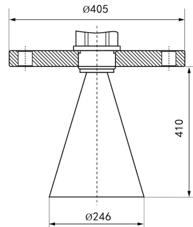
DN250
