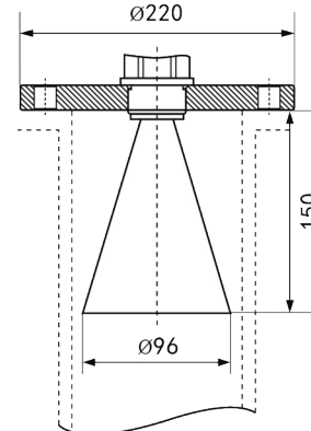
DN250
