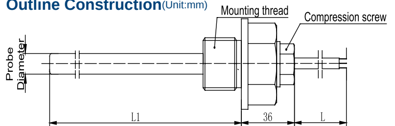
L--Cable version
